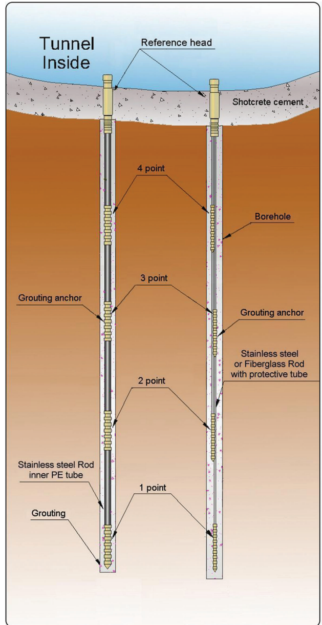
[Installation of mechanical rod extensometer]
