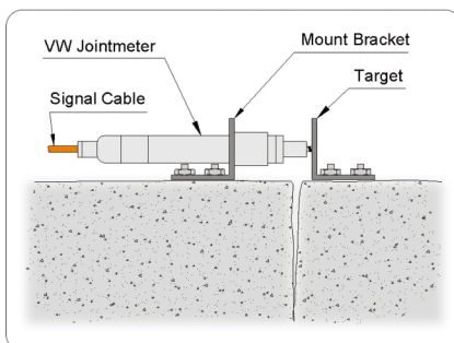
[Uniaxial installation of surface mount jointmeter]
