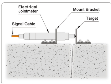
[Uniaxial Installation]
