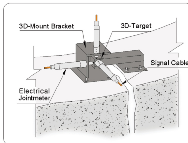
[Triaxial Installation]
