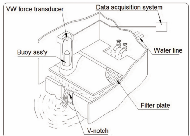
[Installation of VW weir monitoring system]
